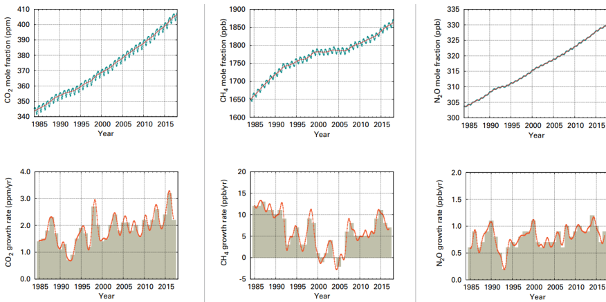
Figure 1 Top row: Globally averaged mole fraction (measure of concentration) from 1984 to 2017 of CO 2 (ppm; left), CH 4 (ppb; center) and N 2 O (ppb; right). The red line is the monthly mean mole fraction with the seasonal variations removed (using global observation data and statistical methods) ; the blue dots and line show the monthly averages. Bottom row: Growth rates representing increases in successive annual means of mole fractions for CO 2 (ppm per year; left), CH 4 (ppb per year; center) and N 2 O (ppb per year; right) (WMO, 2020).
